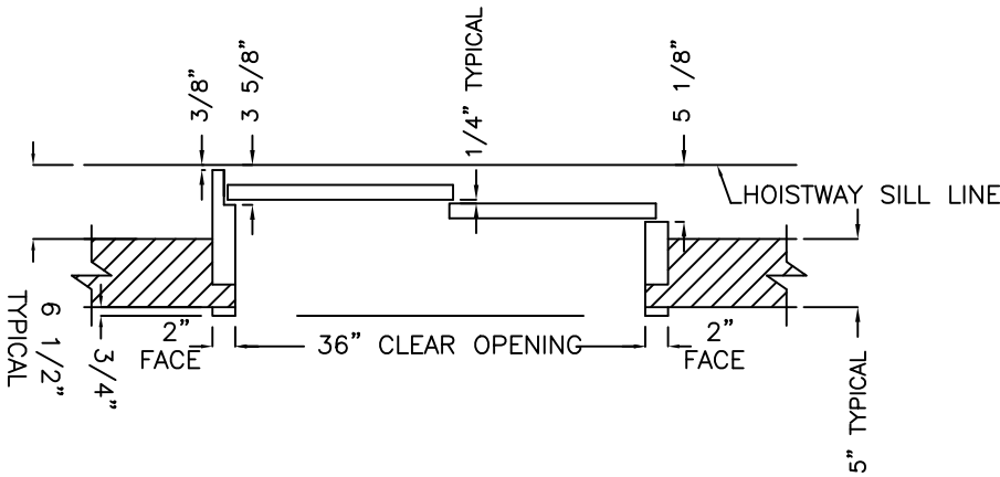
ENTRANCE ELEVATION TWO SPEED LEFT HAND DOOR & ENTRANCE (FRONT)
