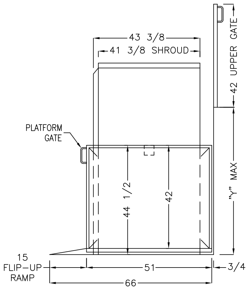
SIDE VIEW
