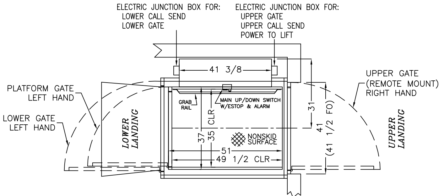
PLAN VIEW
