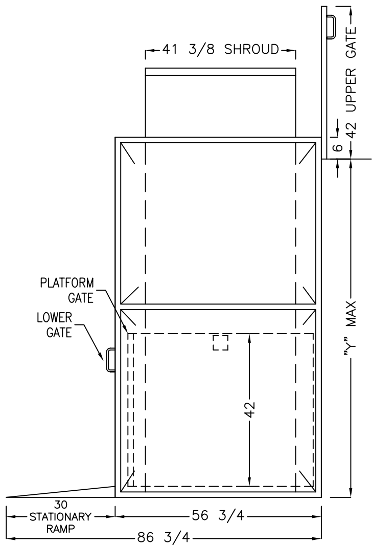
SIDE VIEW
