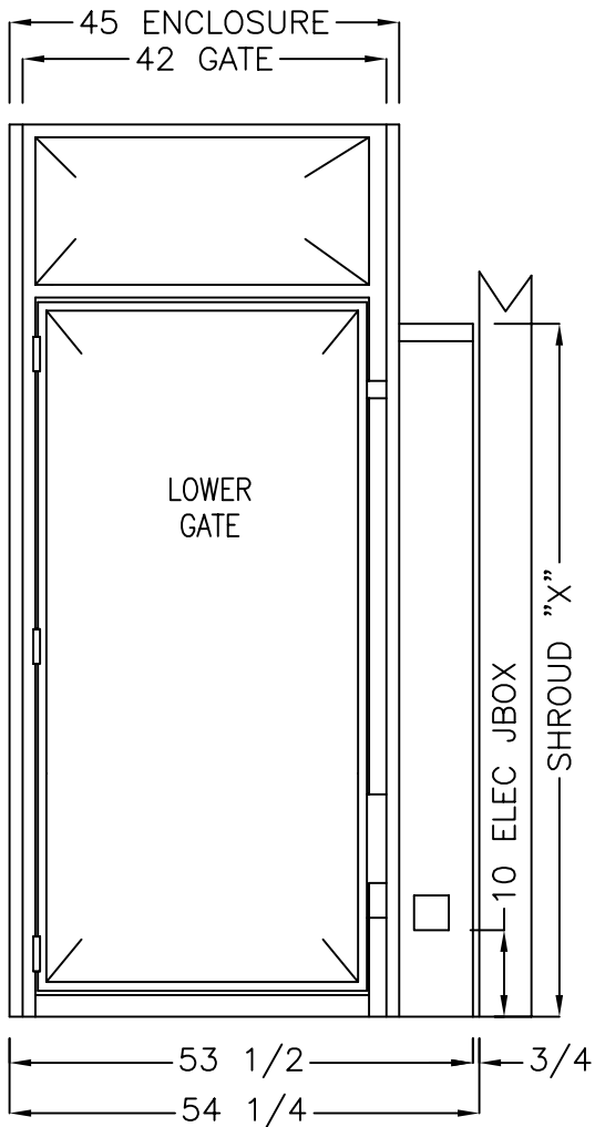
FRONT VIEW
