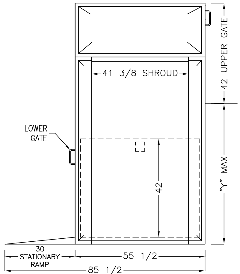
SIDE VIEW
