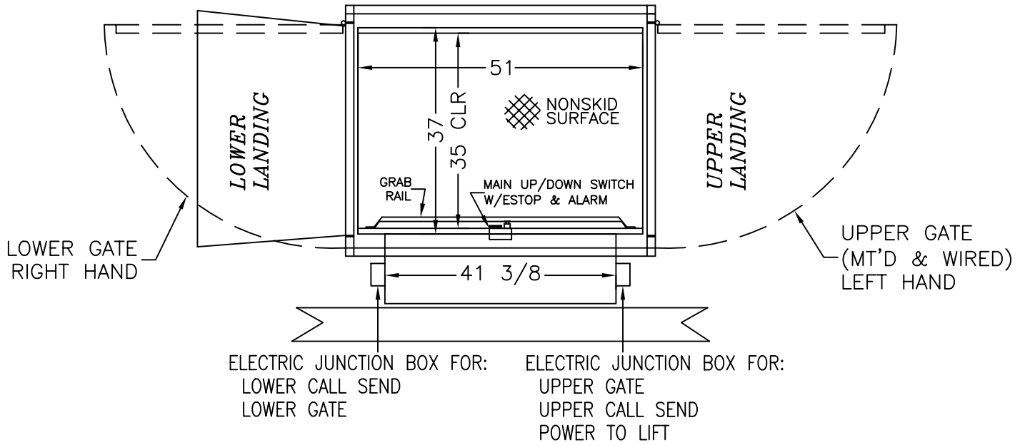
PLAN VIEW
