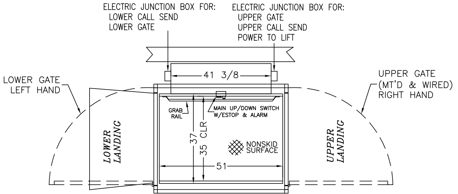
PLAN VIEW
